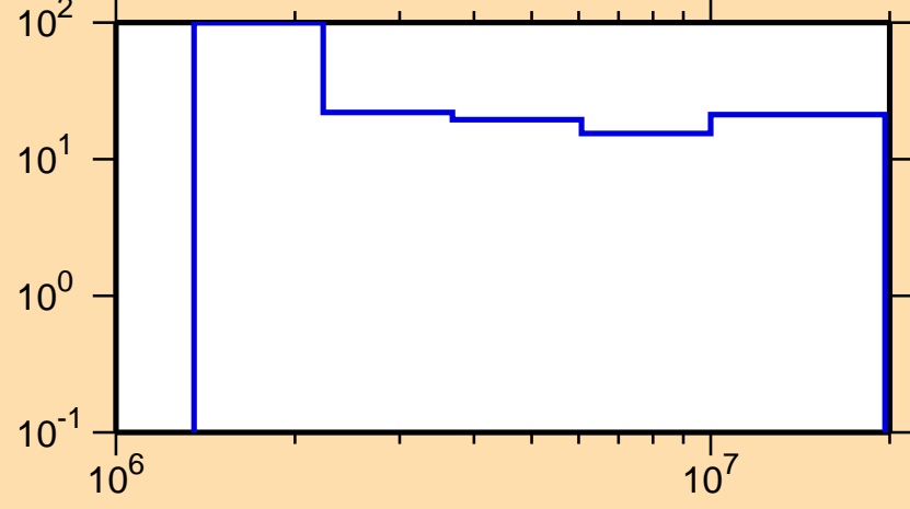
\Delta\sigma/\sigma vs. E for ^{102}\text{Ag}(n,n\text{cont.})
