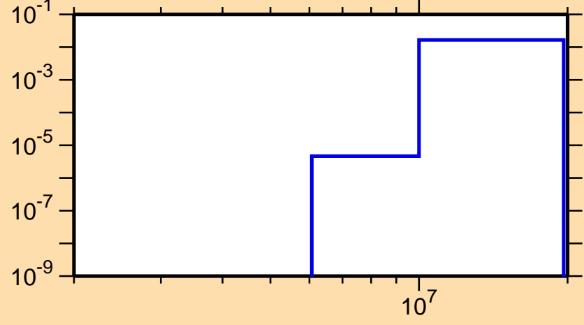
\sigma vs. E for ^{102}\text{Ag}(n,n\alpha)
