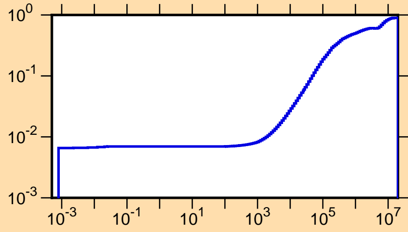
\mu vs. E for ^{103}\text{Ag}(\text{mt251})
