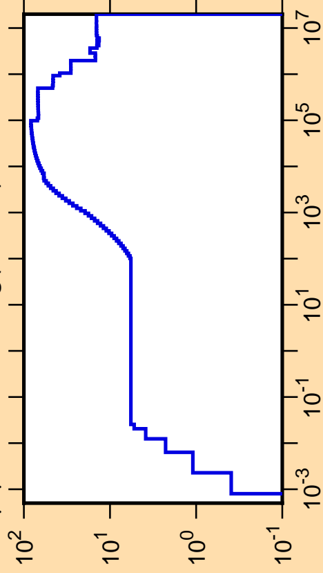
\Delta\mu/\mu vs. E for ^{103}\text{Ag}(\text{mt251})
