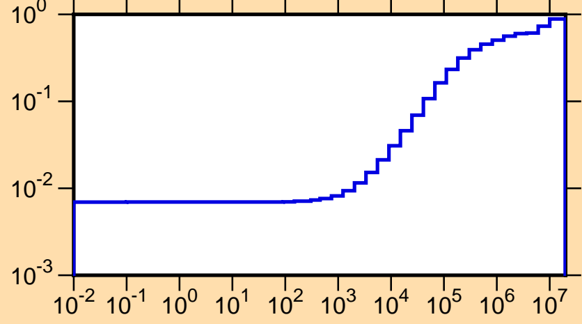
\mu vs. E for ^{103}\text{Ag}(\text{mt251})
