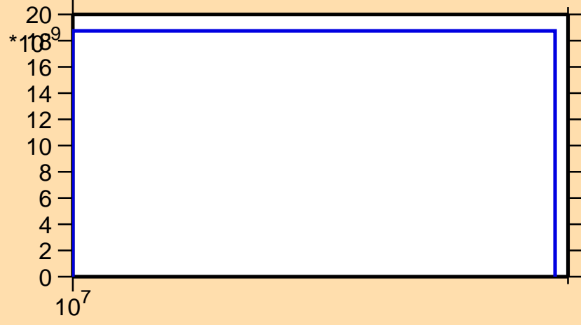
\sigma vs. E for ^{103}\text{Ag}(n,\text{pd})
