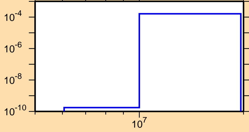
\sigma vs. E for ^{103}\text{Ag}(n,t)
