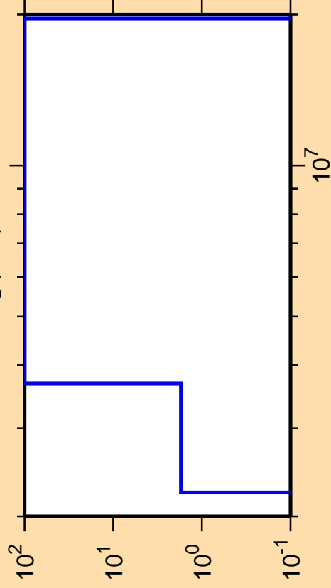
\Delta\sigma/\sigma vs. E for ^{103}\text{Ag}(n,d)
