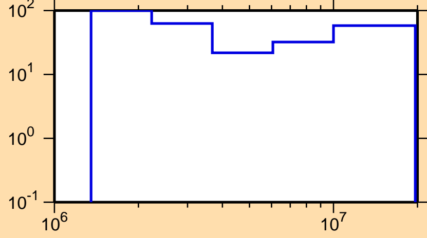
\Delta\sigma/\sigma vs. E for ^{103}\text{Ag}(n,n\text{cont.})
