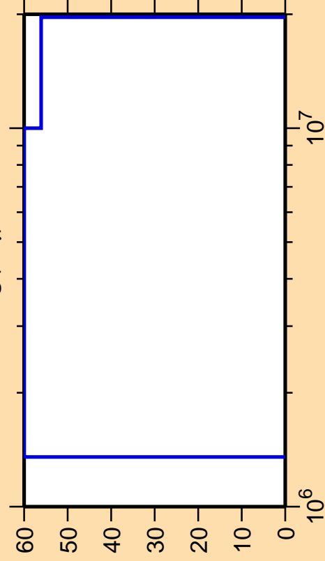
\Delta\sigma/\sigma vs. E for ^{103}\text{Ag}(n,\gamma)
