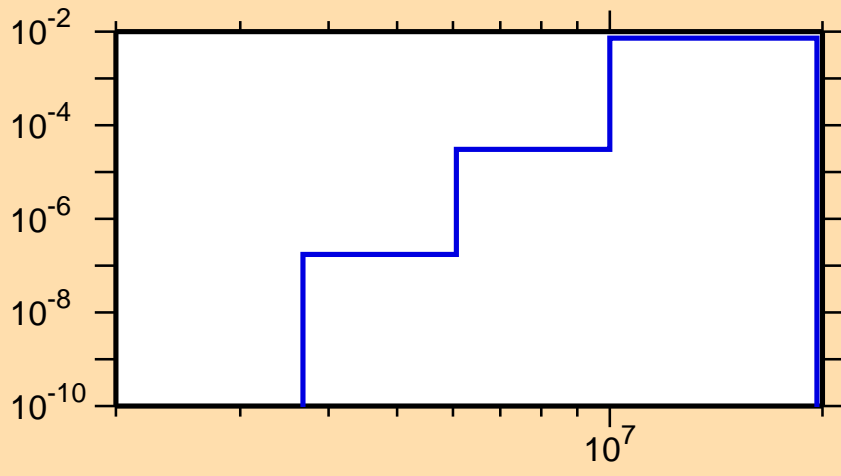
\sigma vs. E for ^{103}\text{Ag}(n,d)
