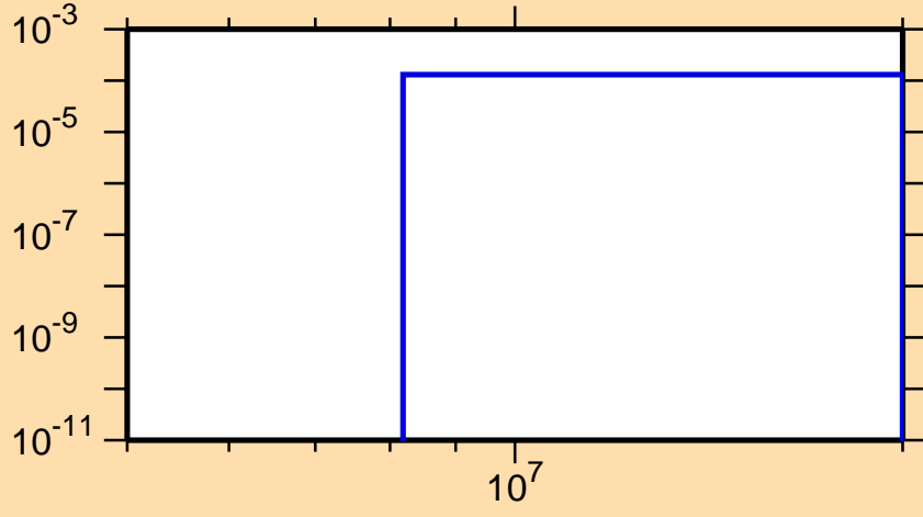
\sigma vs. E for ^{103}\text{Ag}(n,t)
