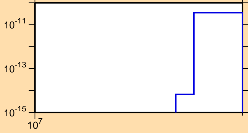
\sigma vs. E for ^{104}\text{Ag}(\text{mt } 34)
