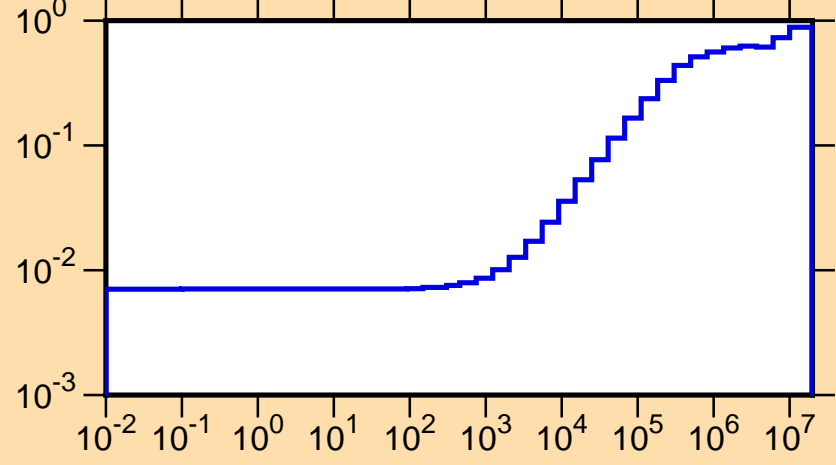
\mu vs. E for ^{104}\text{Ag}(\text{mt251})
