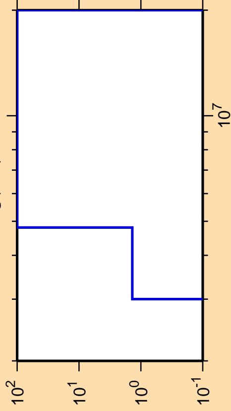
\Delta\sigma/\sigma vs. E for ^{104}\text{Ag}(n,d)
