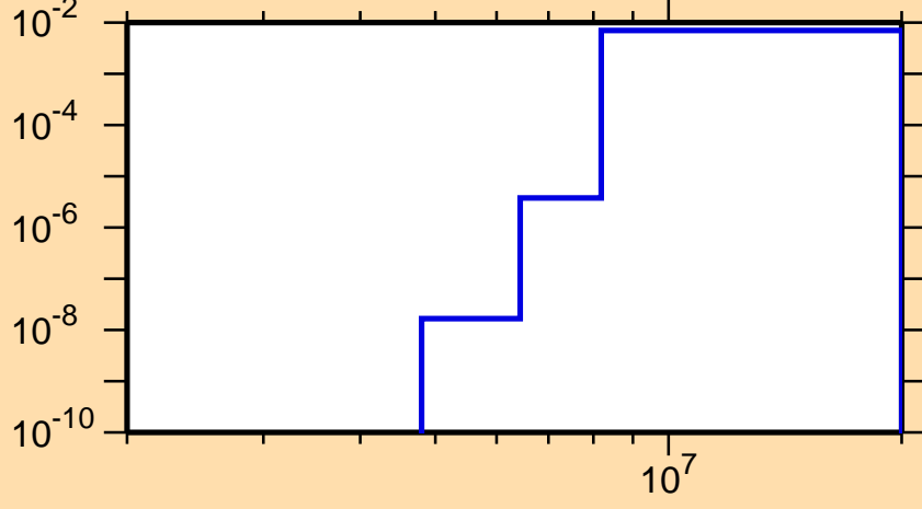
\sigma vs. E for ^{104}\text{Ag}(n,d)
