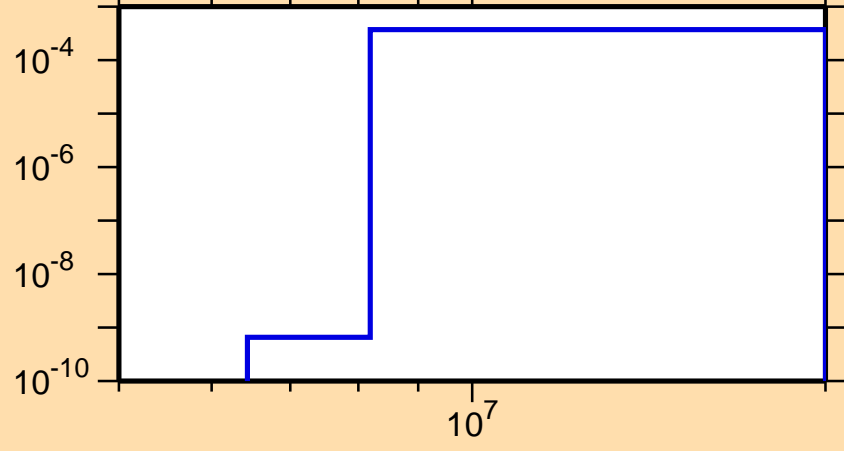
\sigma vs. E for ^{104}\text{Ag}(n,t)
