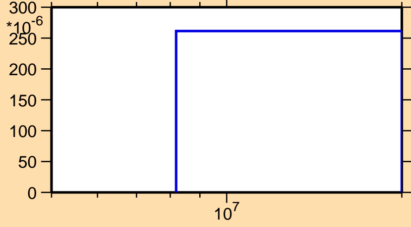
\sigma vs. E for ^{104}\text{Ag}(n,2np)
