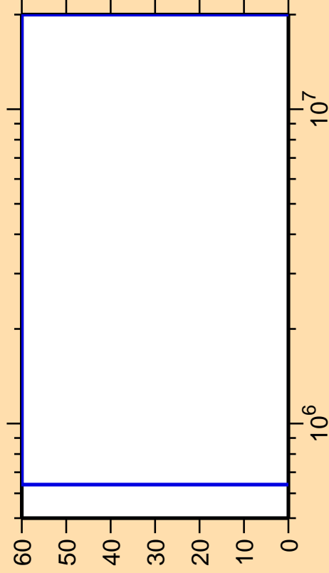
\Delta\sigma/\sigma vs. E for ^{104}\text{Ag}(n,\gamma)
