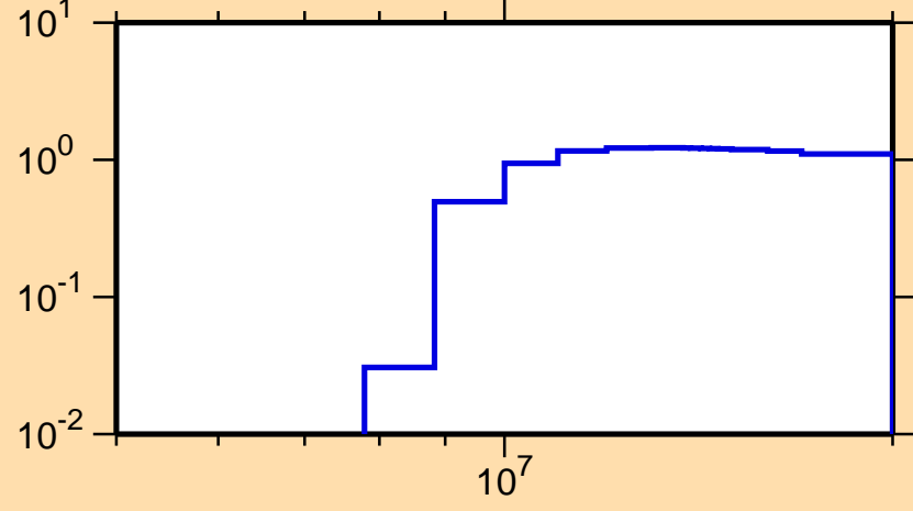
\sigma vs. E for ^{104}\text{Ag}(n,2n)
