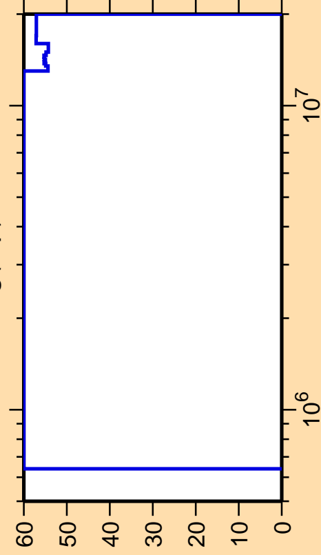
\Delta\sigma/\sigma vs. E for ^{104}\text{Ag}(n,p)
