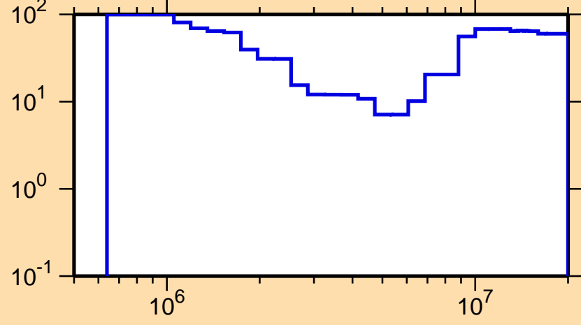
\Delta\sigma/\sigma vs. E for ^{104}\text{Ag}(n,n\text{cont.})
