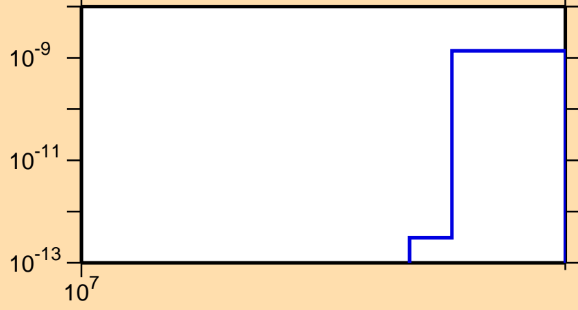
\sigma vs. E for ^{104}\text{Ag}(n,\text{pt})
