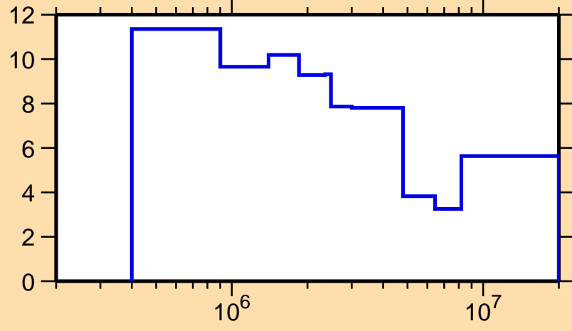
\Delta\sigma/\sigma vs. E for ^{104}\text{Ag}(n,tot.)
