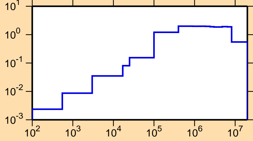
\sigma vs. E for ^{104}\text{Ag}(n,\text{inel.})
