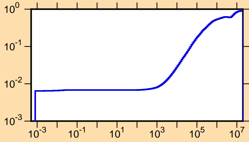
\mu vs. E for ^{105}\text{Ag}(\text{mt251})
