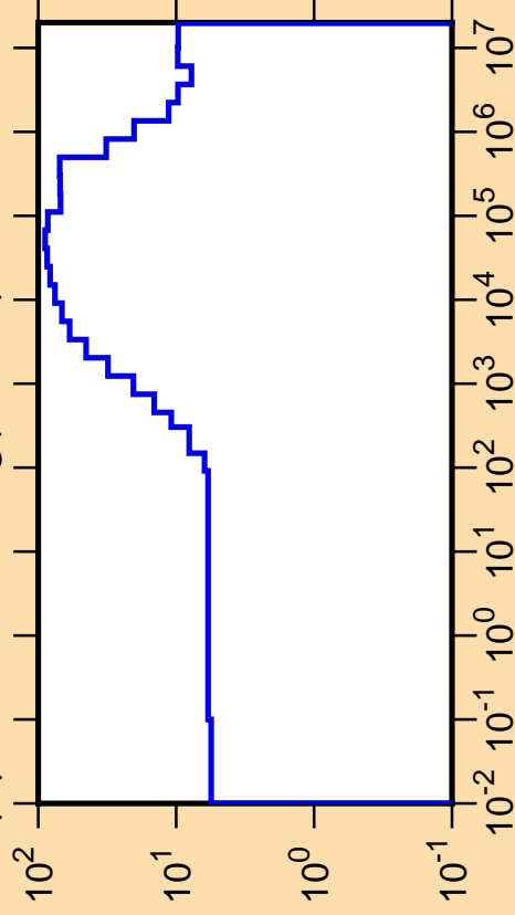
\Delta\mu/\mu vs. E for ^{105}\text{Ag}(\text{mt251})
