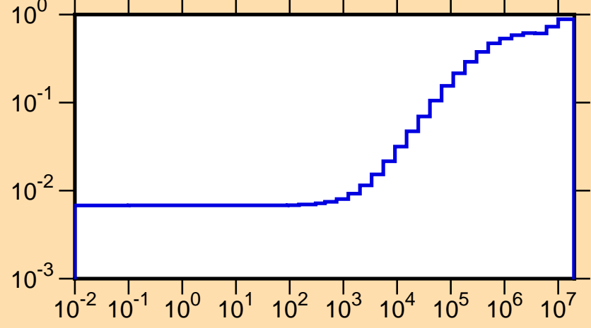
\mu vs. E for ^{105}\text{Ag}(\text{mt251})
