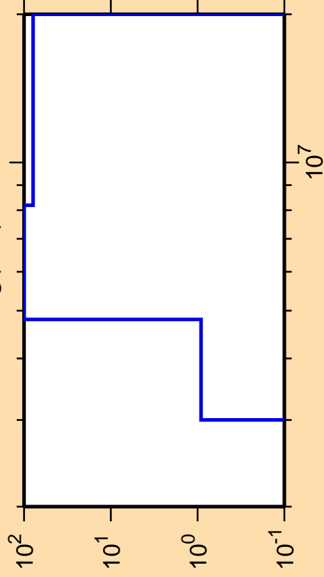
\Delta\sigma/\sigma vs. E for ^{105}\text{Ag}(n,d)
