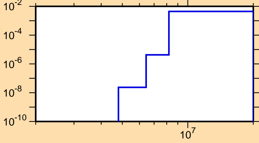
\sigma vs. E for ^{105}\text{Ag}(n,d)
