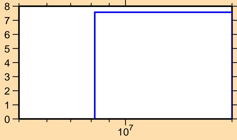
\Delta\sigma/\sigma vs. E for ^{105}\text{Ag}(n,\text{tot.})
