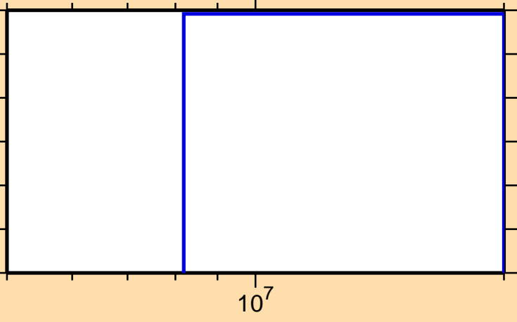
\sigma vs. E for ^{105}\text{Ag}(n,2np)
