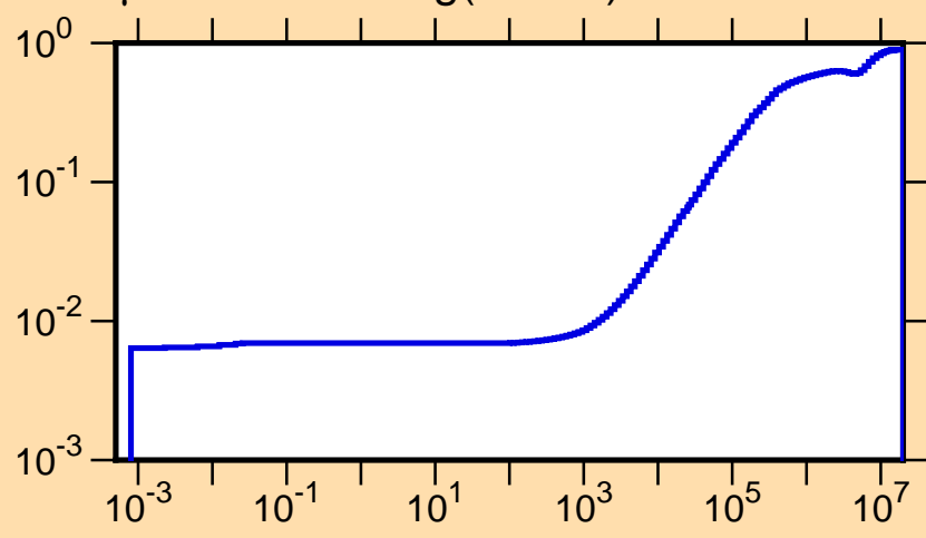
\mu vs. E for ^{106}\text{Ag}(\text{mt251})
