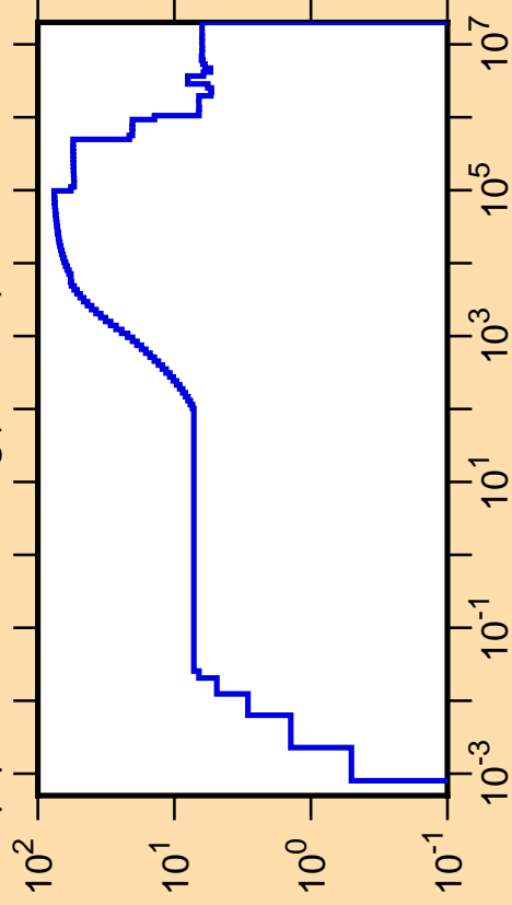
\Delta\mu/\mu vs. E for ^{106}\text{Ag}(\text{mt251})
