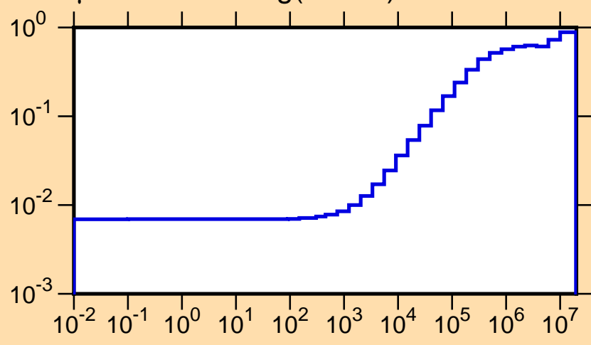
\mu vs. E for ^{106}\text{Ag}(\text{mt251})
