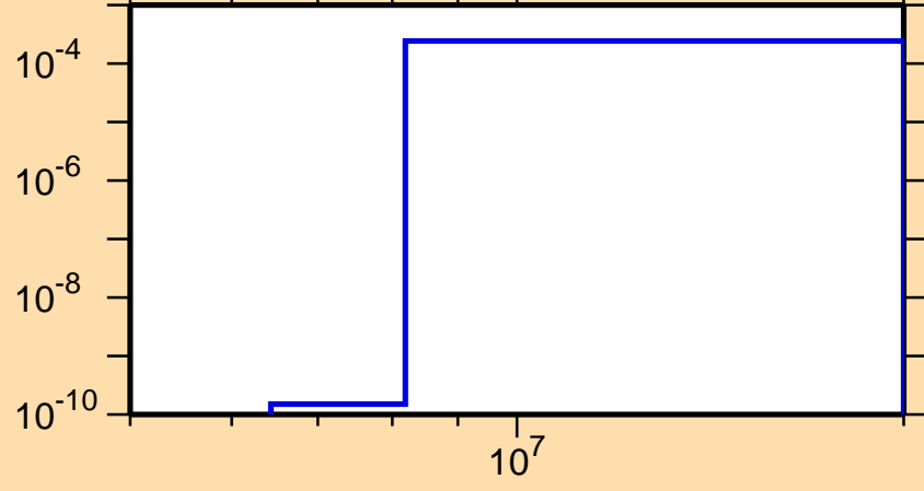
\sigma vs. E for ^{106}\text{Ag}(n,t)
