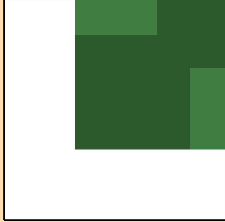
\sigma vs. E for ^{106}\text{Ag}(n,2n)
