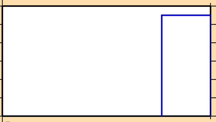
\sigma vs. E for ^{106}\text{Ag}(n,3n)
