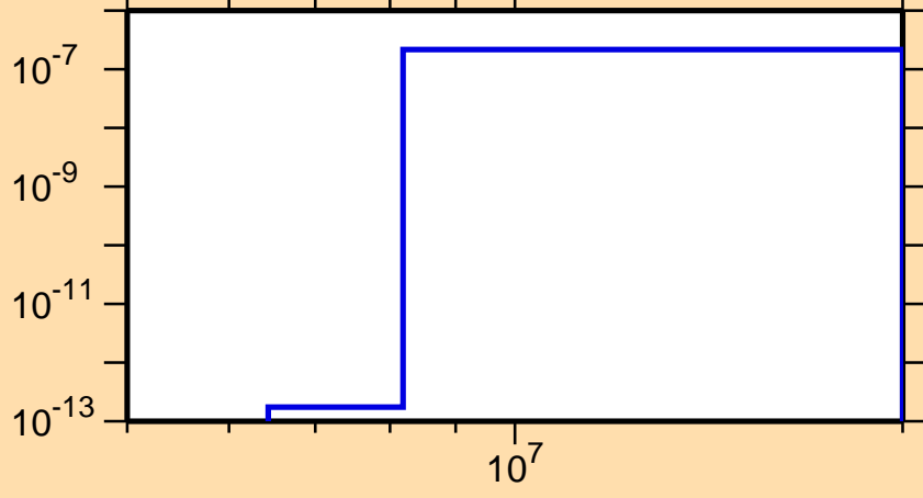
\sigma vs. E for ^{106}\text{Ag}(n,p\alpha)
