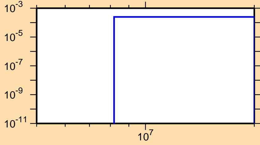
\sigma vs. E for ^{106}\text{Ag}(n,t)
