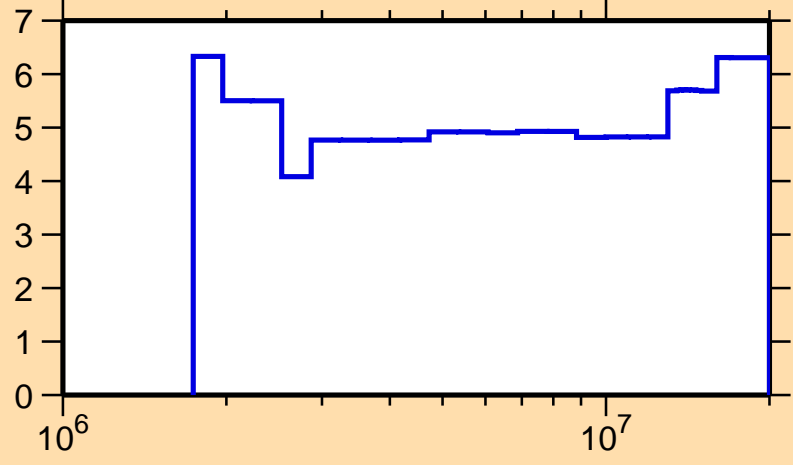
\Delta\sigma/\sigma vs. E for ^{107}\text{Ag}(n,n\text{onel.})
