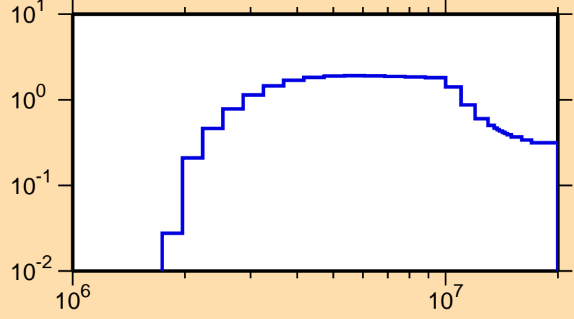
\sigma vs. E for ^{107}\text{Ag}(n,n\text{cont.})
