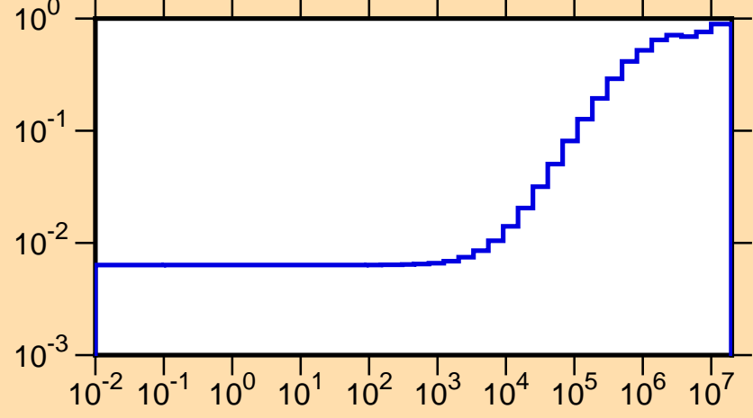
\mu vs. E for ^{107}\text{Ag}(\text{mt251})
