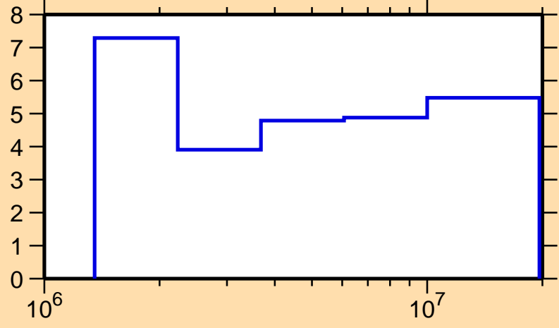
\Delta\sigma/\sigma vs. E for ^{107}\text{Ag}(n,n\text{nonel.})
