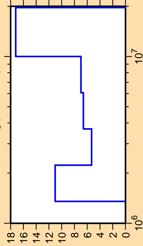
\Delta\sigma/\sigma vs. E for ^{107}\text{Ag}(n,ncont.)
