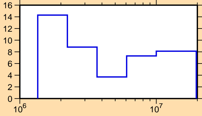
\Delta\sigma/\sigma vs. E for ^{107}\text{Ag}(n,el.)
