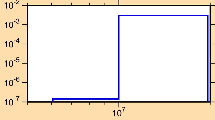
\sigma vs. E for ^{107}\text{Ag}(n,n\alpha)
