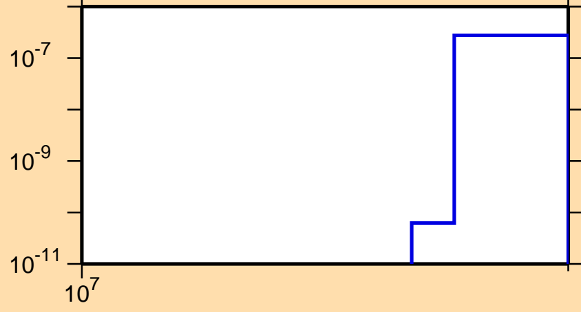
\sigma vs. E for ^{108}\text{Ag}(n,nt)
