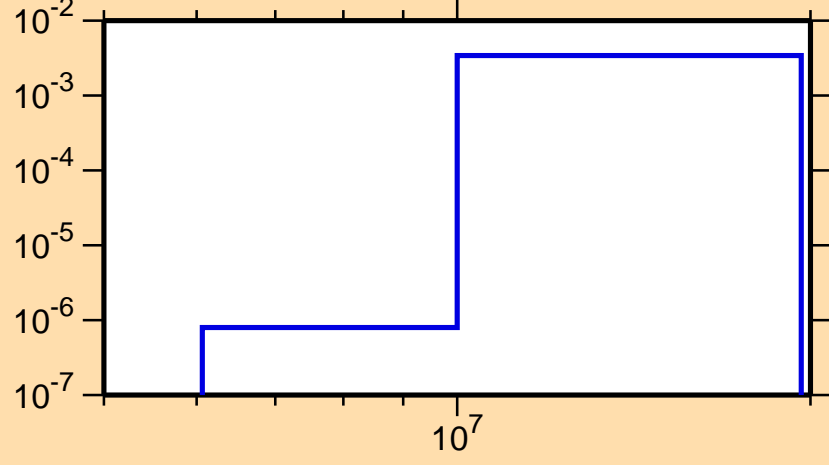
\sigma vs. E for ^{108}\text{Ag}(n,d)
