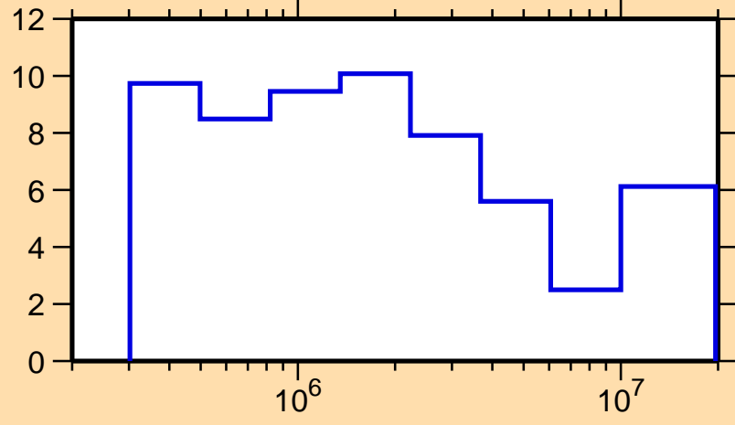
\Delta\sigma/\sigma vs. E for ^{108}\text{Ag}(n,tot.)
