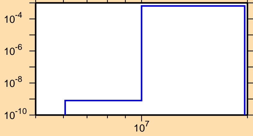
\sigma vs. E for ^{108}\text{Ag}(n,n\alpha)
