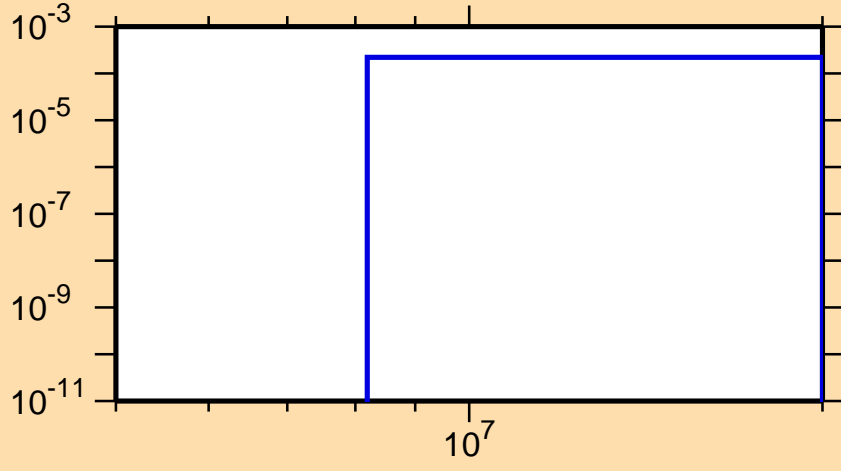
\sigma vs. E for ^{108}\text{Ag}(n,t)
