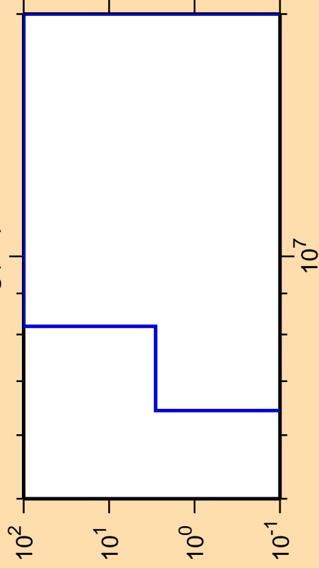
\Delta\sigma/\sigma vs. E for ^{108}\text{Ag}(n,t)
