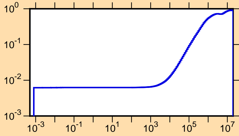
\mu vs. E for ^{109}\text{Ag}(\text{mt251})
