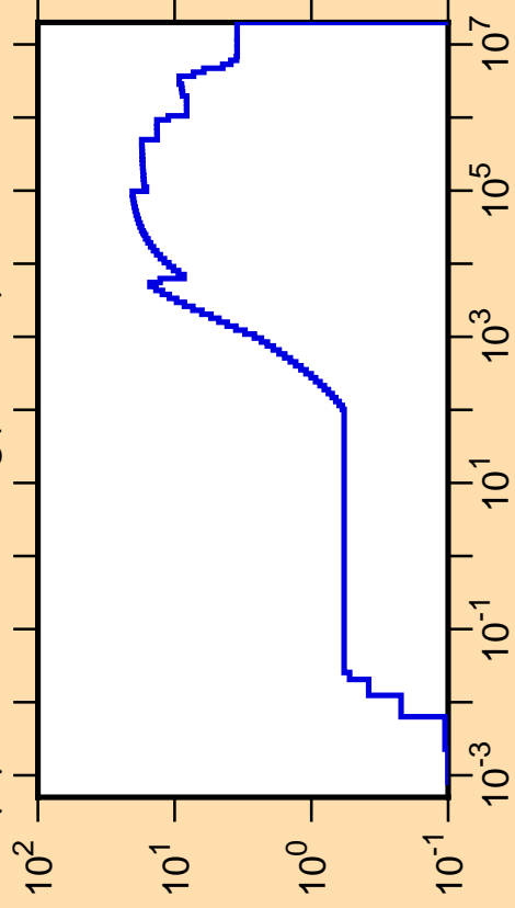
\Delta\mu/\mu vs. E for ^{109}\text{Ag}(\text{mt251})
