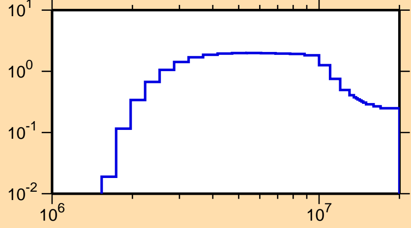
\sigma vs. E for ^{109}\text{Ag}(n,n\text{cont.})
