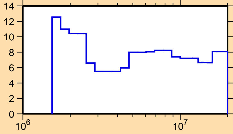
\Delta\sigma/\sigma vs. E for ^{109}\text{Ag}(n,n\text{nonel.})
