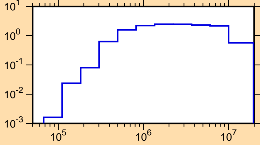
\sigma vs. E for ^{109}\text{Ag}(n,\text{inel.})
