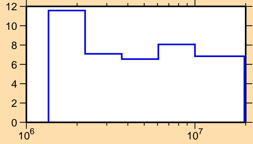
\Delta\sigma/\sigma vs. E for ^{109}\text{Ag}(n,n\text{inel.})
