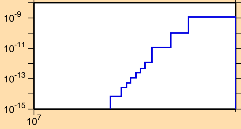
\sigma vs. E for ^{109}\text{Ag}(n,p\alpha)
