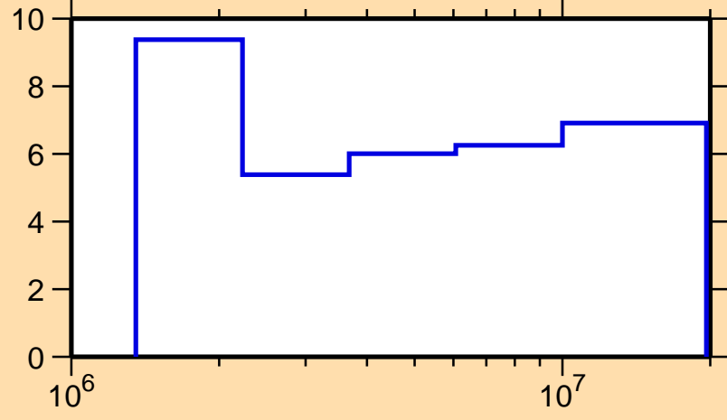
\Delta\sigma/\sigma vs. E for ^{109}\text{Ag}(n,n\text{onel.})
