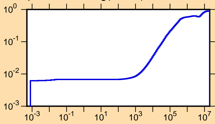
\mu vs. E for ^{110}\text{Ag}(\text{mt251})
