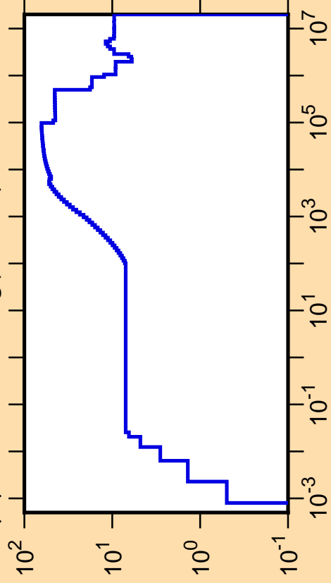
\Delta\mu/\mu vs. E for ^{110}\text{Ag}(\text{mt251})
