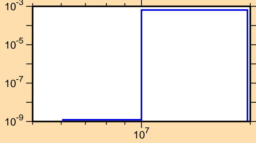
\sigma vs. E for ^{110}\text{Ag}(n,t)
