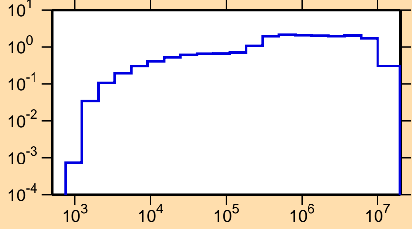
\sigma vs. E for ^{110}\text{Ag}(n,\text{inel.})
