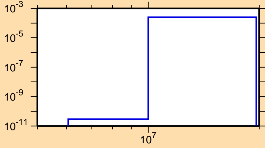
\sigma vs. E for ^{110}\text{Ag}(n,n\alpha)
