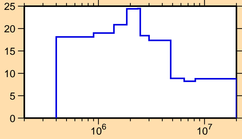
\Delta\sigma/\sigma vs. E for ^{110}\text{Ag}(n,el.)
