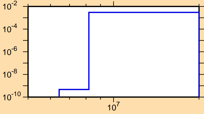
\sigma vs. E for ^{110}\text{Ag}(n,d)
