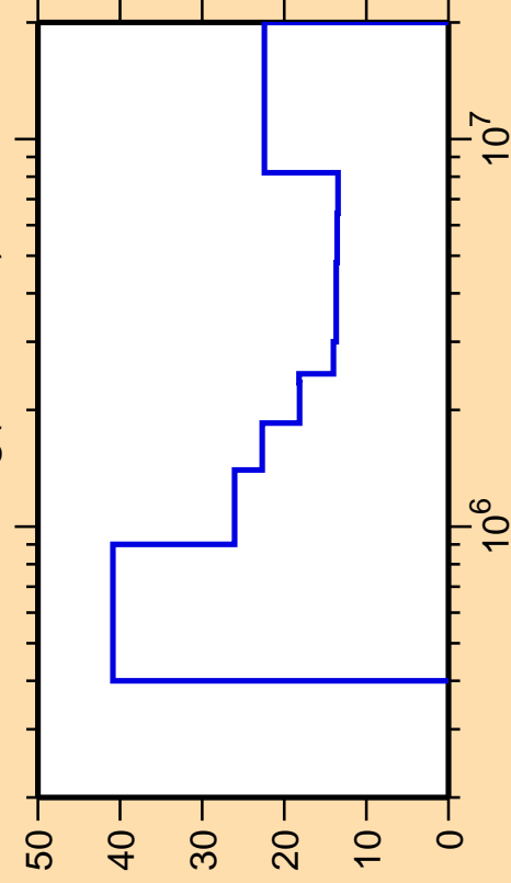
\Delta\sigma/\sigma vs. E for ^{110}\text{Ag}(n,ncont.)
