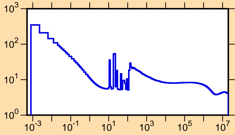
\sigma vs. E for ^{110}\text{Ag}(n,\text{tot.})
