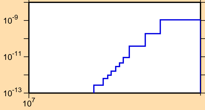
\sigma vs. E for ^{110}\text{Ag}(n,p\alpha)
