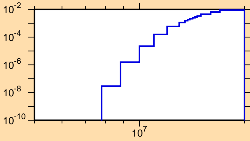
\sigma vs. E for ^{110}\text{Ag}(n,d)
