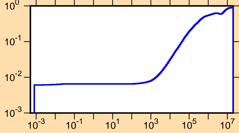
\mu vs. E for ^{111}\text{Ag}(\text{mt251})
