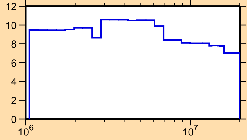
\Delta\sigma/\sigma vs. E for ^{111}\text{Ag}(n,n\text{onel.})
