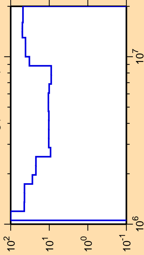
\Delta\sigma/\sigma vs. E for ^{111}\text{Ag}(n,\text{ncont.})
