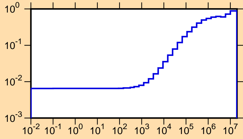
\mu vs. E for ^{111}\text{Ag}(\text{mt251})
