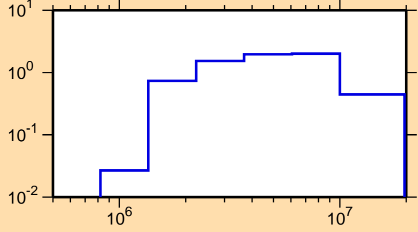
\sigma vs. E for ^{111}\text{Ag}(n,n\text{cont.})
