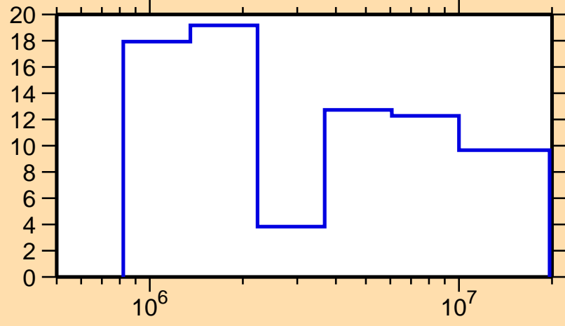
\Delta\sigma/\sigma vs. E for ^{111}\text{Ag}(n,el.)
