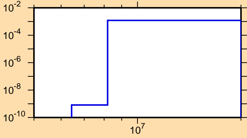
\sigma vs. E for ^{111}\text{Ag}(n,d)
