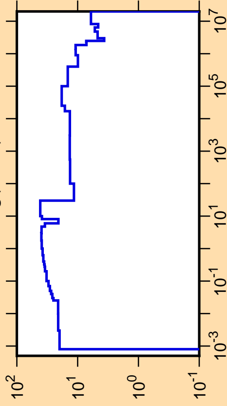
\Delta\sigma/\sigma vs. E for ^{111}\text{Ag}(n,\text{tot.})
