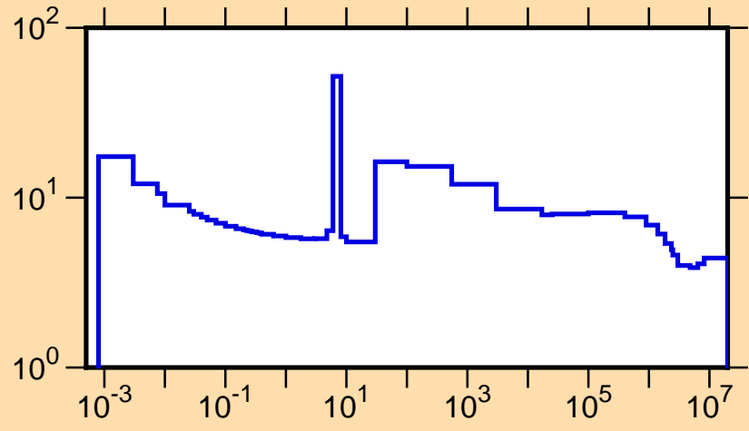
\sigma vs. E for ^{111}\text{Ag}(n,\text{tot.})
