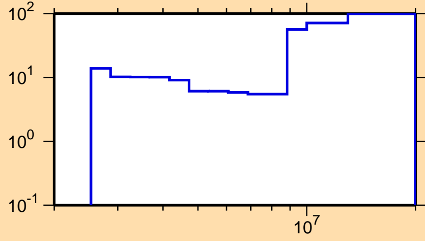
\Delta\sigma/\sigma vs. E for ^{111}\text{Ag}(n,ncont.)
