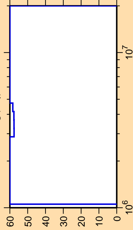
\Delta\sigma/\sigma vs. E for ^{111}\text{Ag}(n,\gamma)
