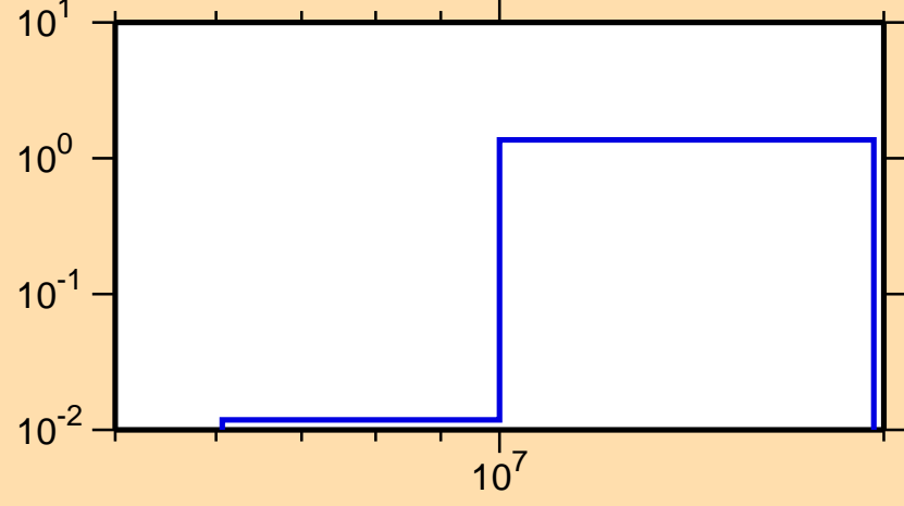
\sigma vs. E for ^{111}\text{Ag}(n,2n)
