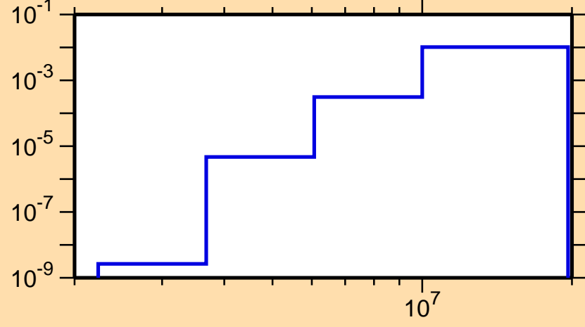
\sigma vs. E for ^{111}\text{Ag}(n,p)
