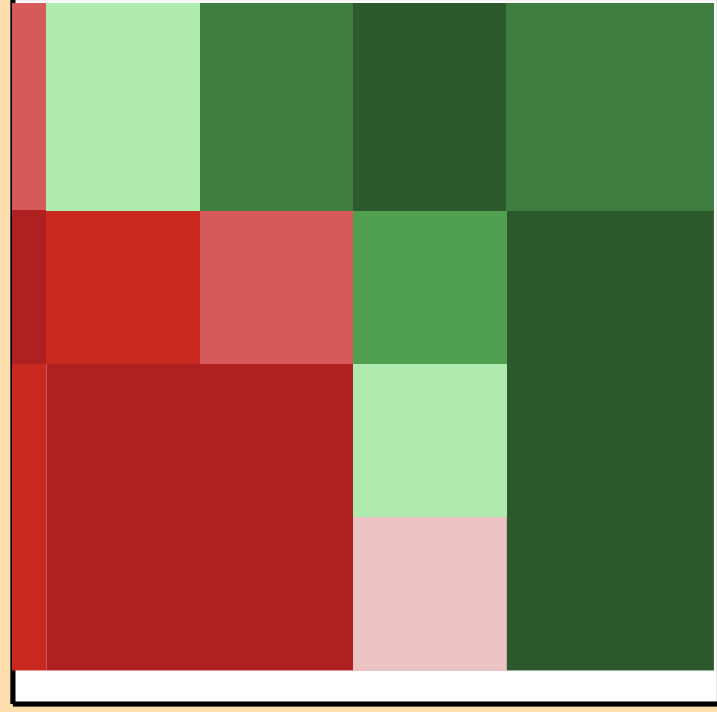
\Delta\sigma/\sigma vs. E for ^{111}\text{Ag}(n,n\text{cont.})
