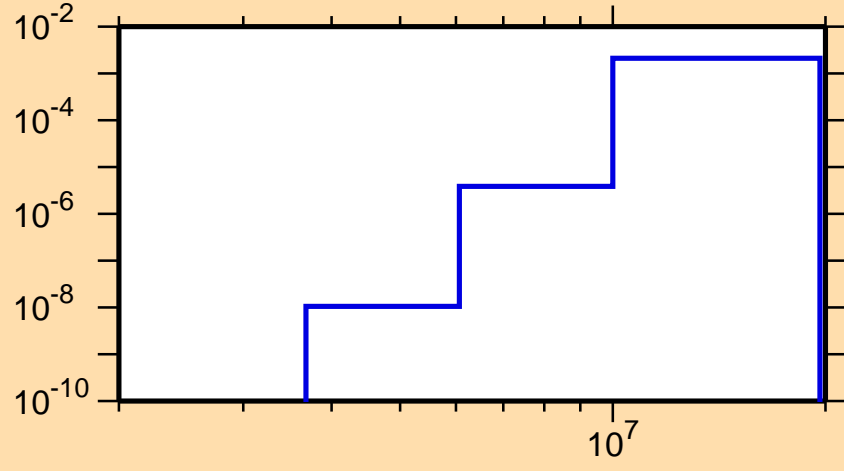
\sigma vs. E for ^{111}\text{Ag}(n,\alpha)
