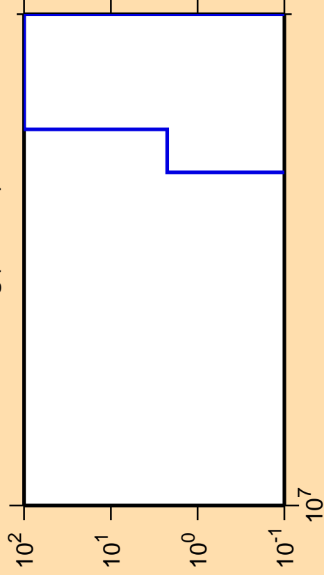
\Delta\sigma/\sigma vs. E for ^{112}\text{Ag}(n,\text{He3})
