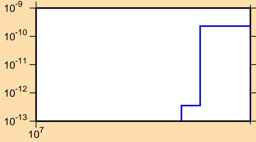
\sigma vs. E for ^{112}\text{Ag}(n,\text{He3})
