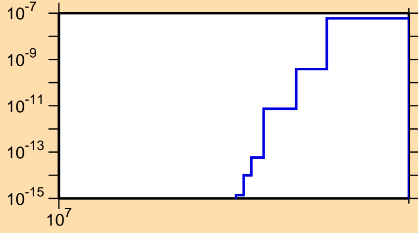
\sigma vs. E for ^{112}\text{Ag}(n,2n\alpha)
