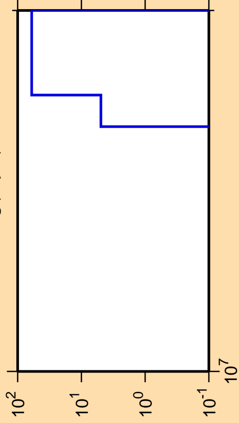
\Delta\sigma/\sigma vs. E for ^{112}\text{Ag}(n,p\alpha)
