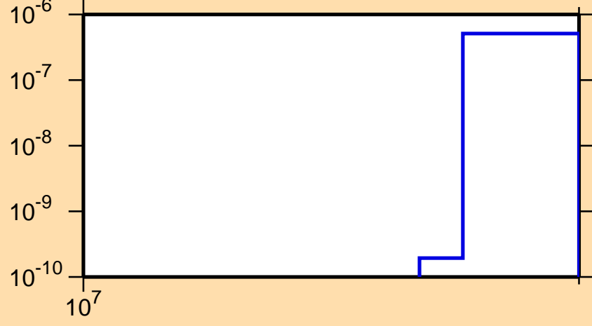
\sigma vs. E for ^{112}\text{Ag}(n,nt)
