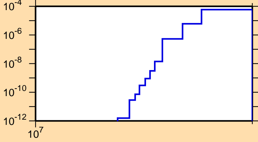
\sigma vs. E for ^{112}\text{Ag}(n,\text{nd})
