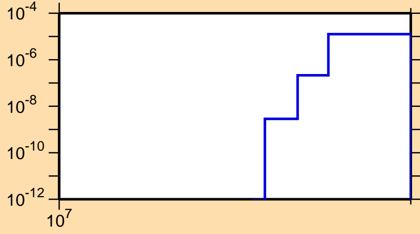
\sigma vs. E for ^{112}\text{Ag}(n,2np)
