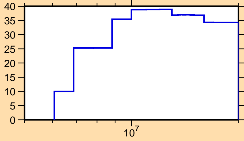
\Delta\sigma/\sigma vs. E for ^{112}\text{Ag}(n,\text{inel.})
