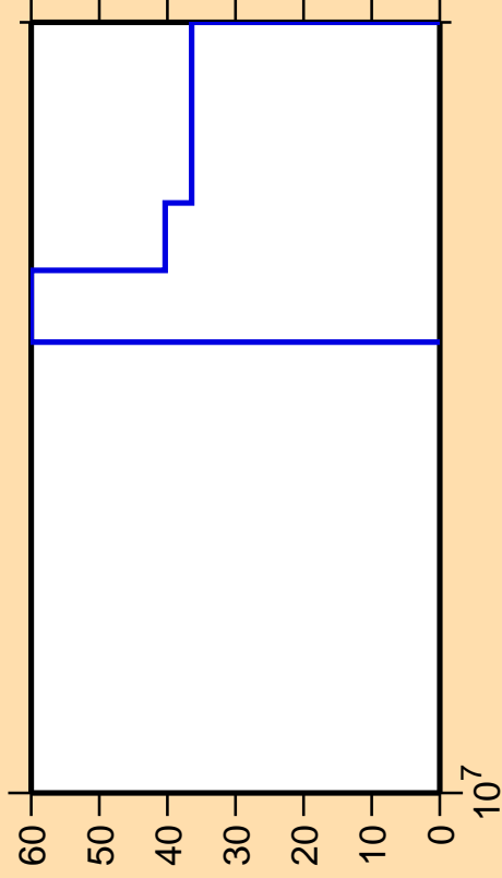
\Delta\sigma/\sigma vs. E for ^{112}\text{Ag}(n,3n)
