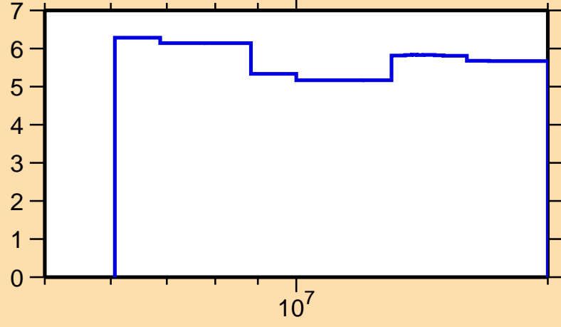
\Delta\sigma/\sigma vs. E for ^{112}\text{Ag}(n,\text{nonel.})
