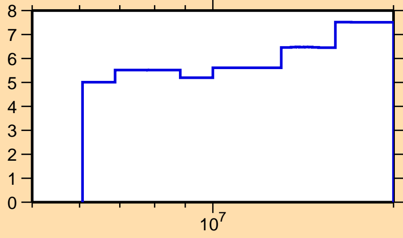
\Delta\sigma/\sigma vs. E for ^{112}\text{Ag}(n,\text{tot.})
