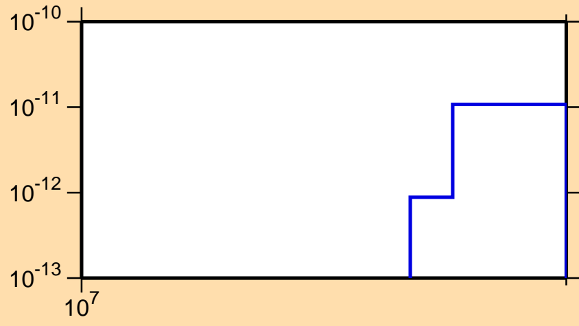
\sigma vs. E for ^{112}\text{Ag}(n,p\alpha)
