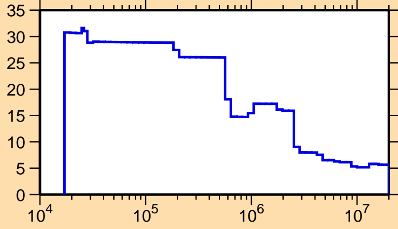
\Delta\sigma/\sigma vs. E for ^{112}\text{Ag}(n,\text{nonel.})
