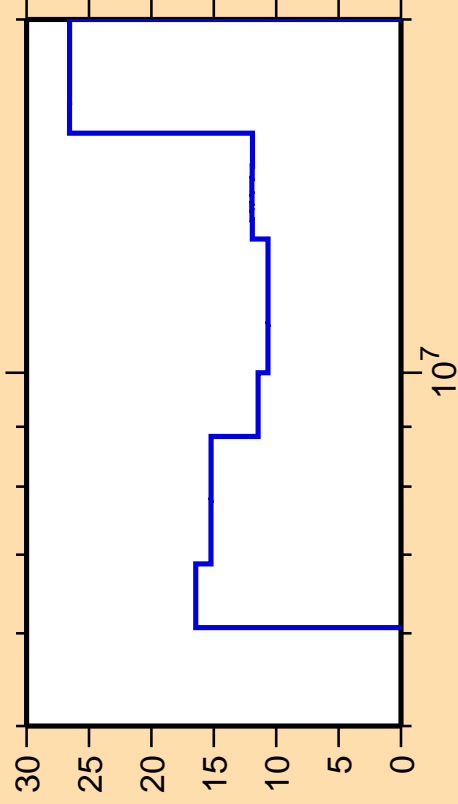
\Delta\sigma/\sigma vs. E for ^{112}\text{Ag}(n,2n)
