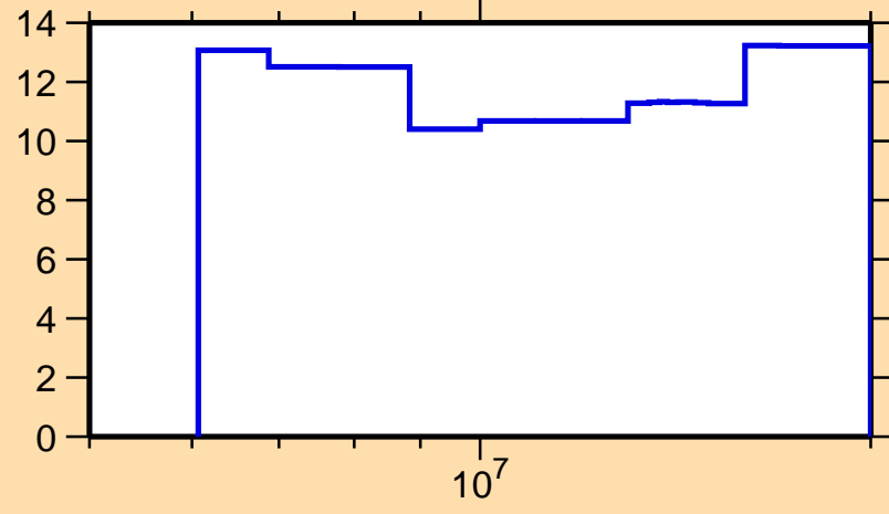
\Delta\sigma/\sigma vs. E for ^{112}\text{Ag}(n,\text{el.})
