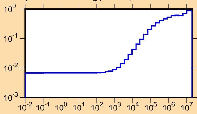
\mu vs. E for ^{112}\text{Ag}(\text{mt251})
