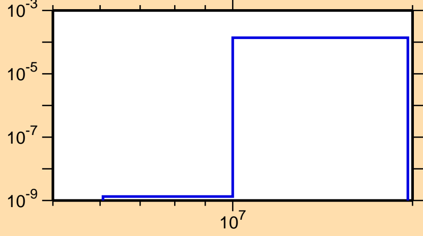
\sigma vs. E for ^{112}\text{Ag}(n,t)
