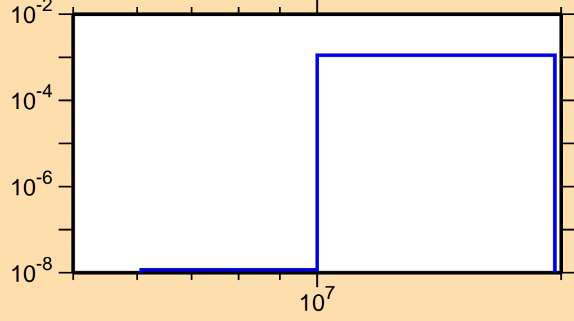
\sigma vs. E for ^{112}\text{Ag}(n,d)
