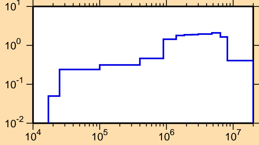
\sigma vs. E for ^{112}\text{Ag}(n,\text{inel.})
