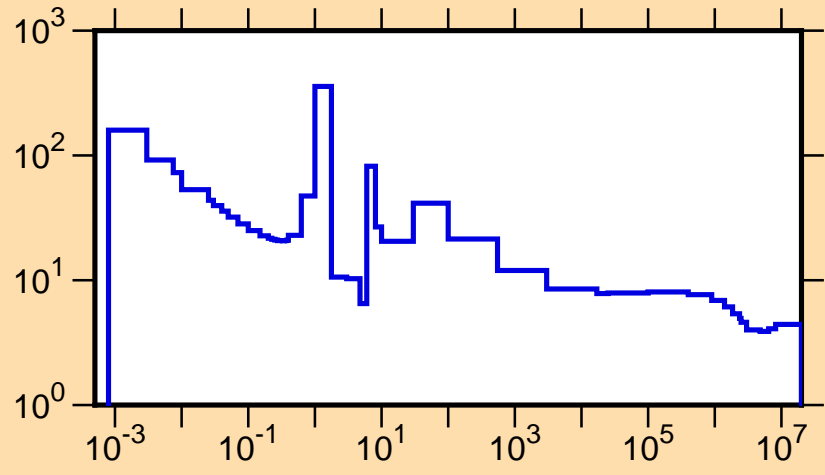
\sigma vs. E for ^{112}\text{Ag}(n,\text{tot.})
