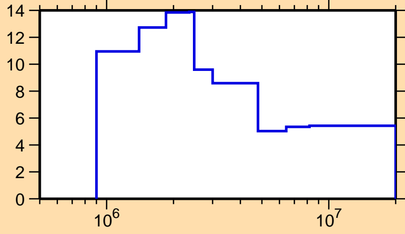
\Delta\sigma/\sigma vs. E for ^{112}\text{Ag}(n,tot.)
