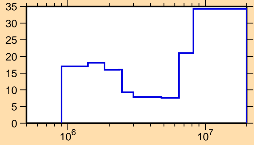
\Delta\sigma/\sigma vs. E for ^{112}\text{Ag}(n,inel.)
