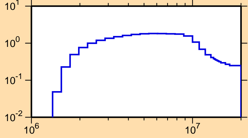
\sigma vs. E for ^{113}\text{Ag}(n,n\text{cont.})
