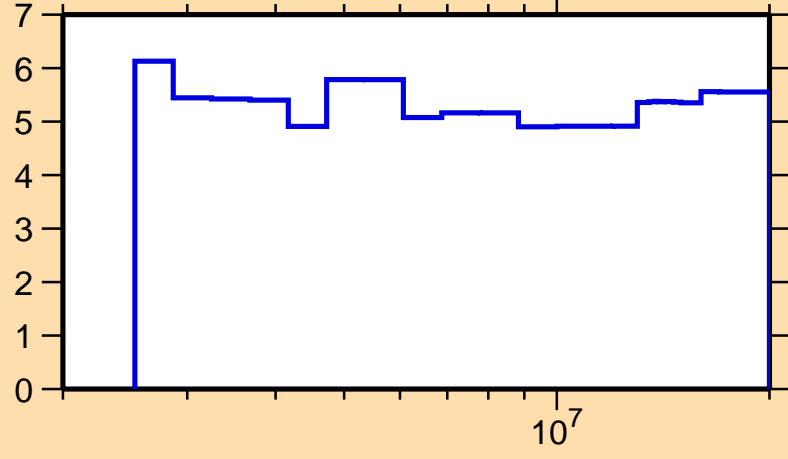
\Delta\sigma/\sigma vs. E for ^{113}\text{Ag}(n,\text{nonel.})
