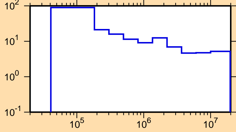
\Delta\sigma/\sigma vs. E for ^{113}\text{Ag}(n,\text{nonel.})
