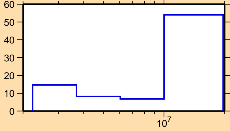
\Delta\sigma/\sigma vs. E for ^{113}\text{Ag}(n,ncont.)
