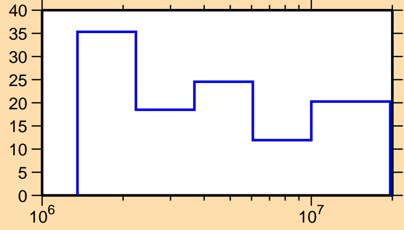
\Delta\sigma/\sigma vs. E for ^{113}\text{Ag}(n,el.)
