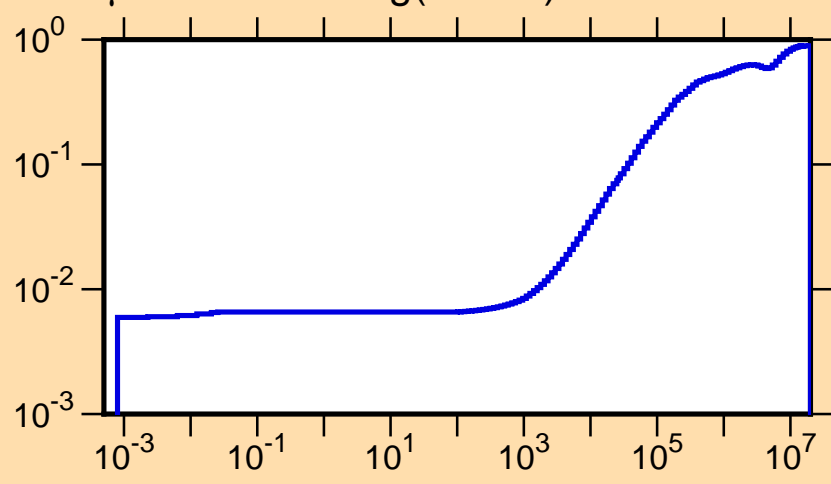
\mu vs. E for ^{114}\text{Ag}(\text{mt251})
