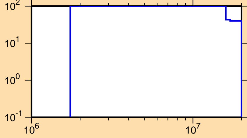
\Delta\sigma/\sigma vs. E for ^{114}\text{Ag}(n,n_1)
