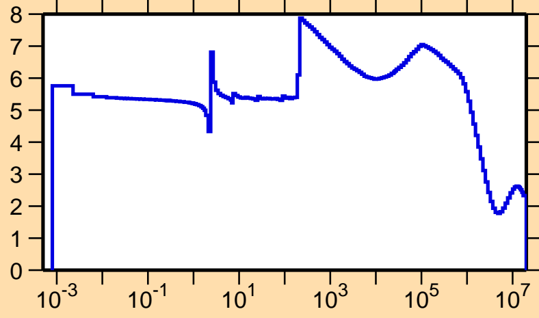
\sigma vs. E for ^{114}\text{Ag}(n,\text{el.})
