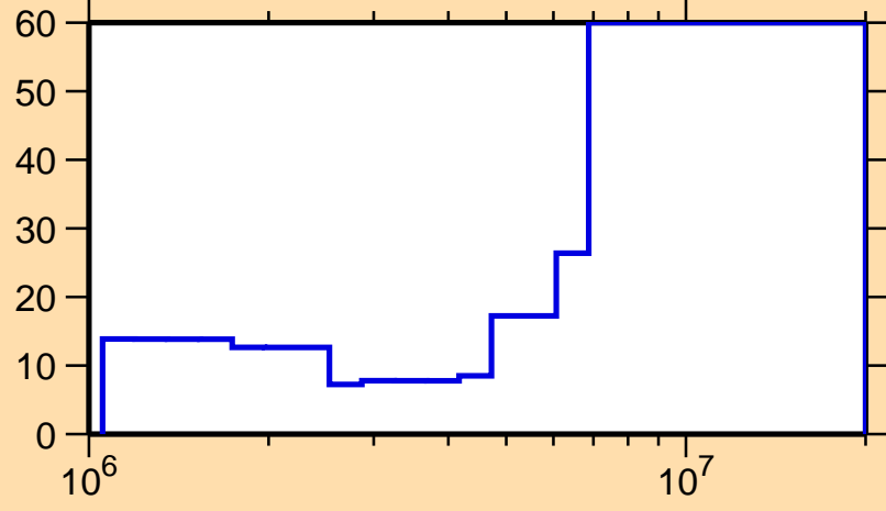
\Delta\sigma/\sigma vs. E for ^{114}\text{Ag}(n,inel.)
