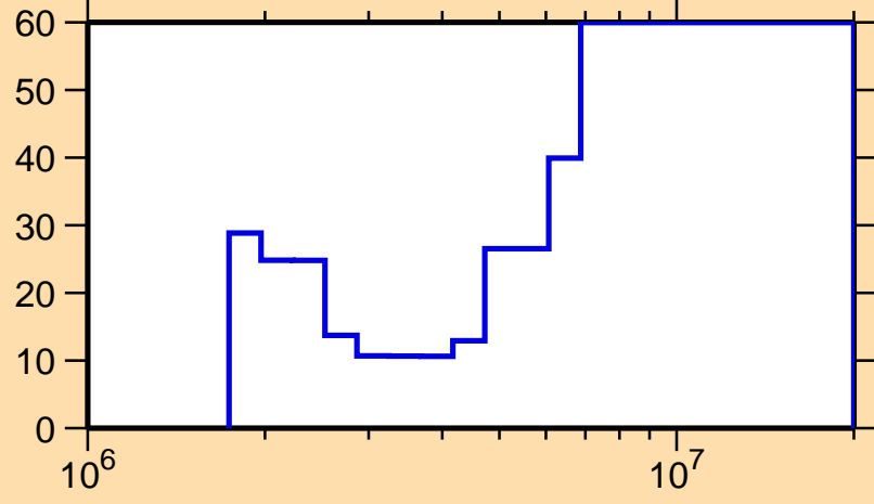
\Delta\sigma/\sigma vs. E for ^{114}\text{Ag}(n,ncont.)
